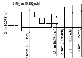
Terminal Dimensions
